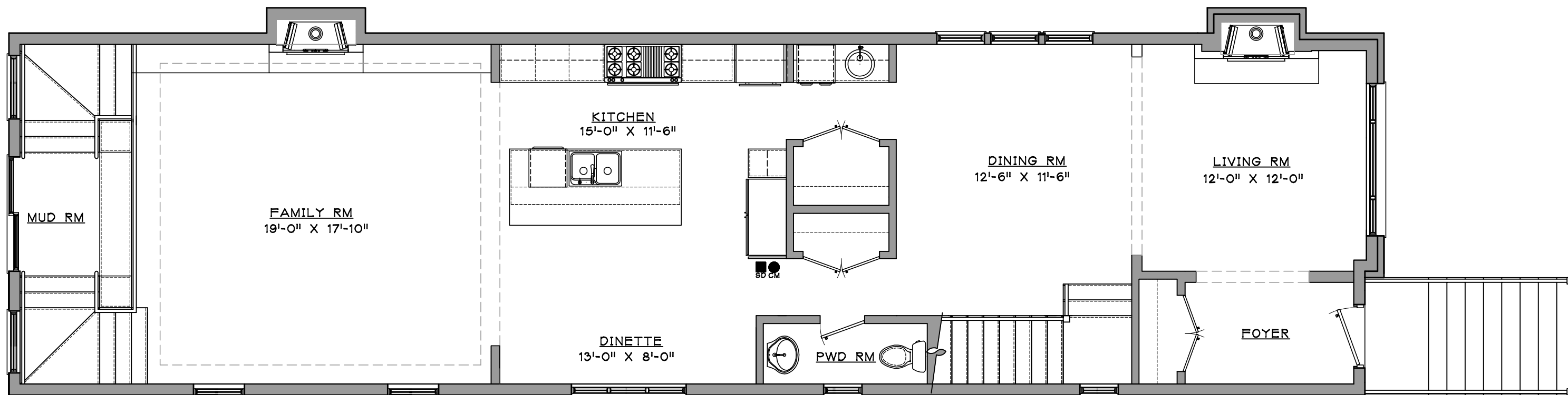
2 FIRST FLOOR PLAN
