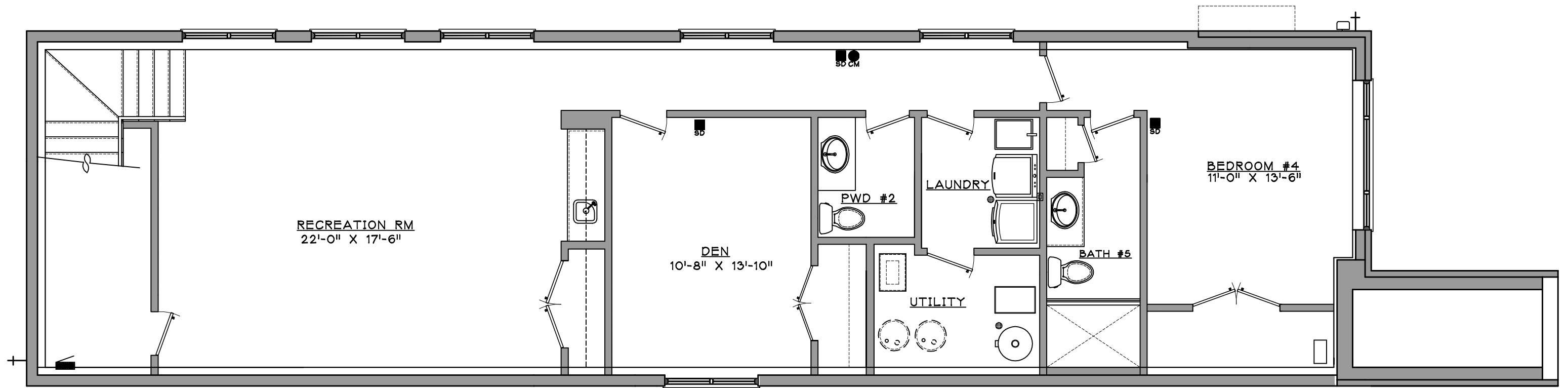
1 LOWER LEVEL PLAN
