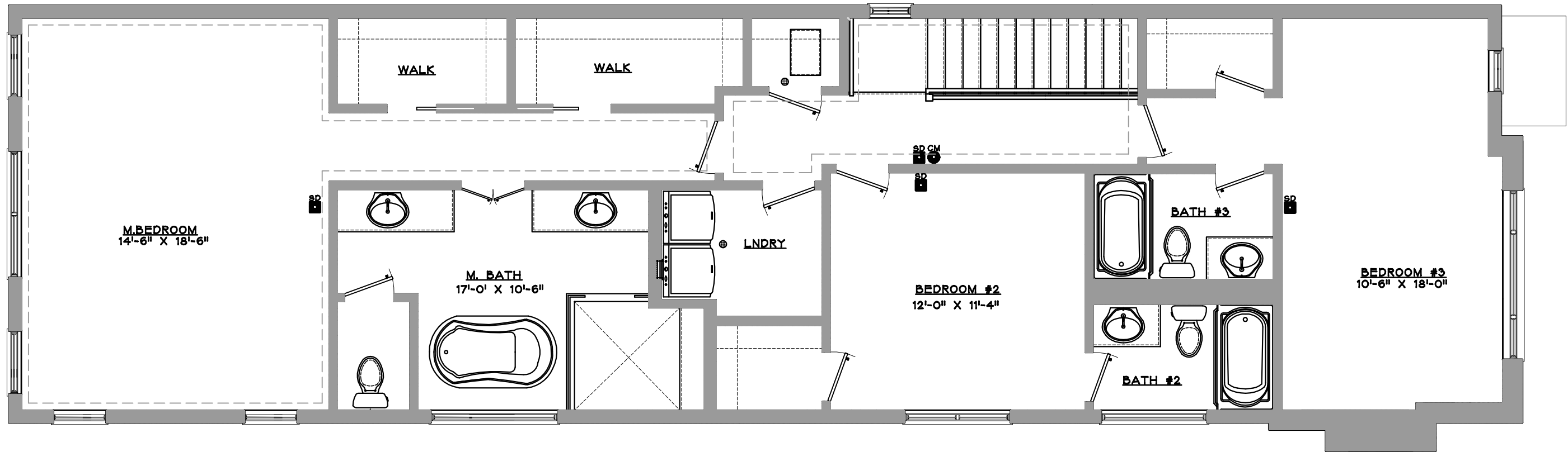
3 SECOND FLOOR PLAN
